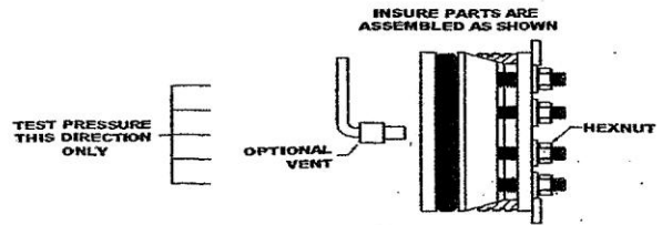
8" Test Plugs
